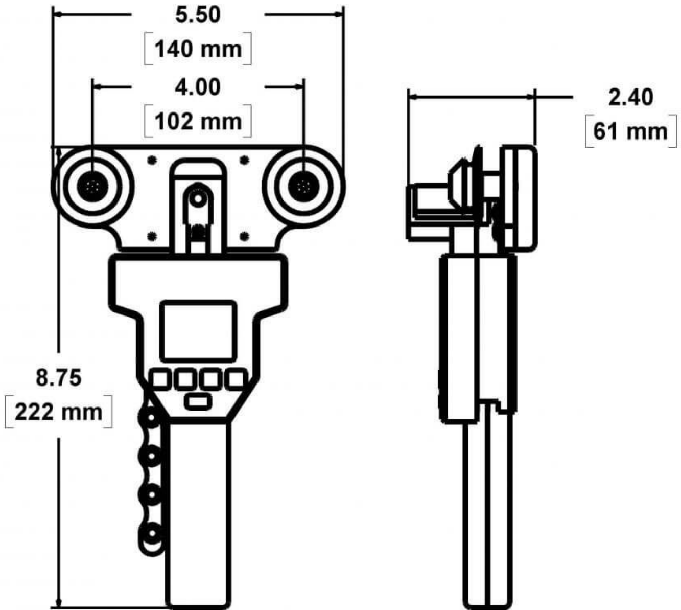
LX-250-1 DIGITAL CABLE TENSION METER (All Models: LX-250-1 and LX-500-1)
